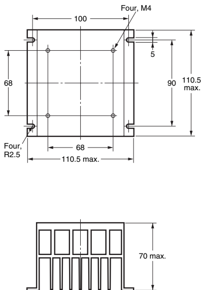
Mounting Holes
