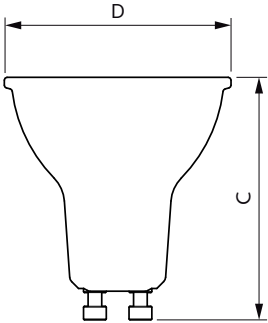
GU10 220-240V 7-100W 730lm 60D 6500K ND
